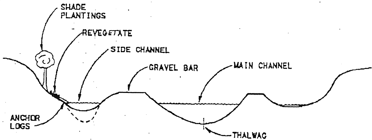
OFF CHANNEL PONDS TYPICAL SECTION A-A
