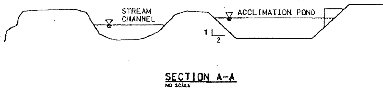
PANTHER CREEK ACCLIMATION POND
